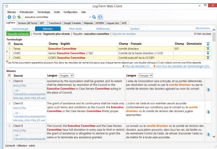
Interface LogiTerm Web Client
